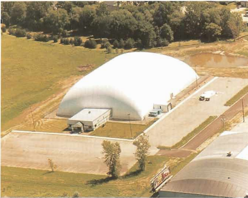
Yeadon® Golf Dome 160' x 210' x 65' high – 34 Tees
