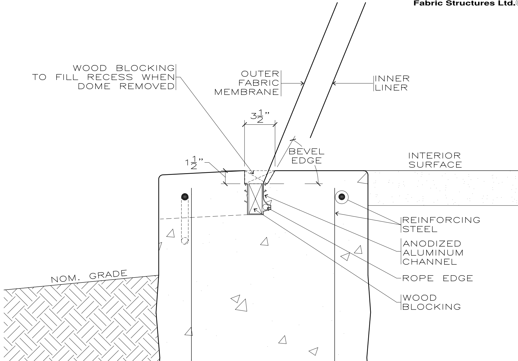
Typical Section Through Grade Beam - Recessed Channel Detail
