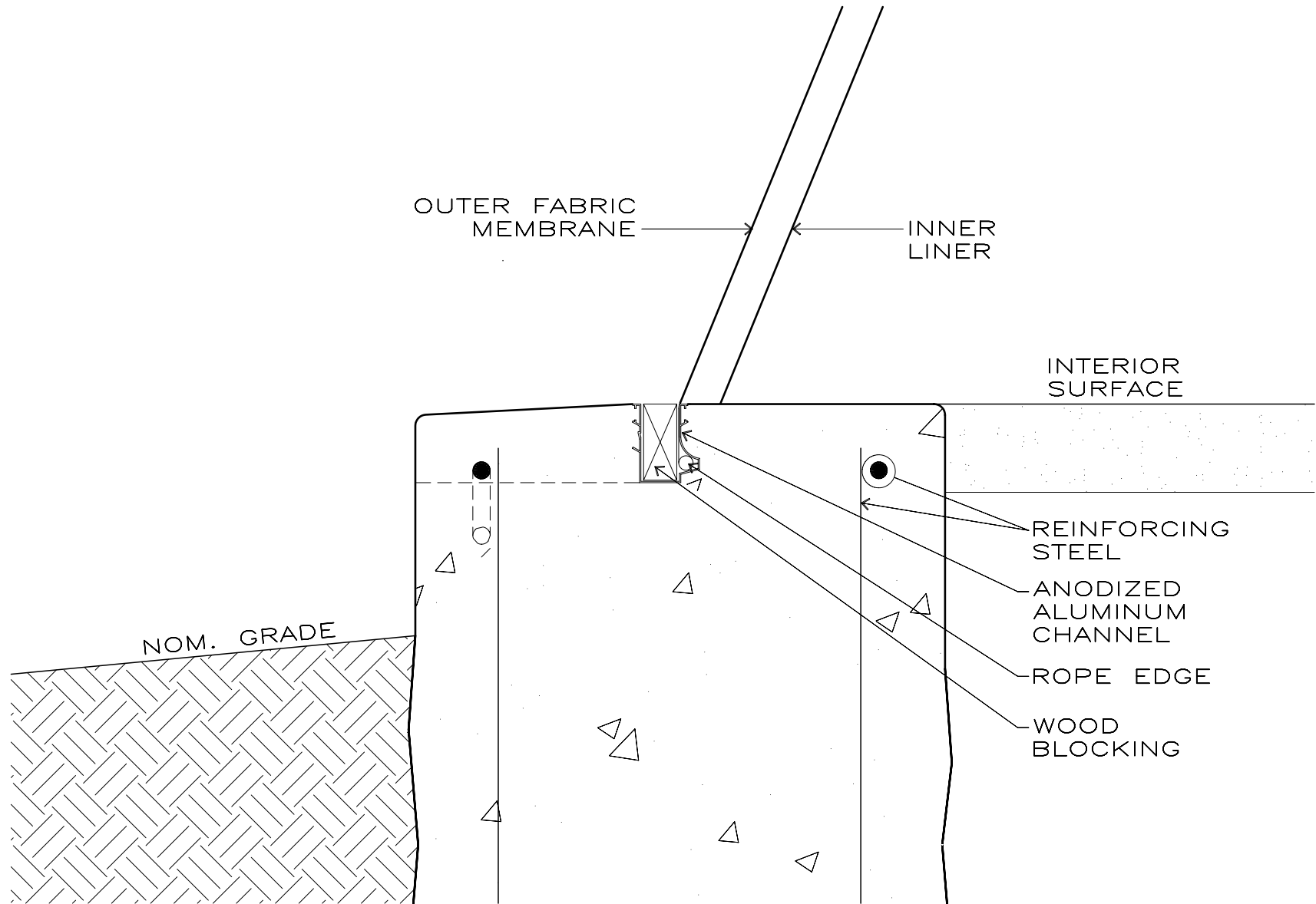
Typical Section Through Grade Beam - Flush Channel Detail
